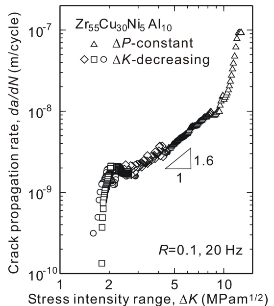
Fig. 1. Crack propagation behavior.
